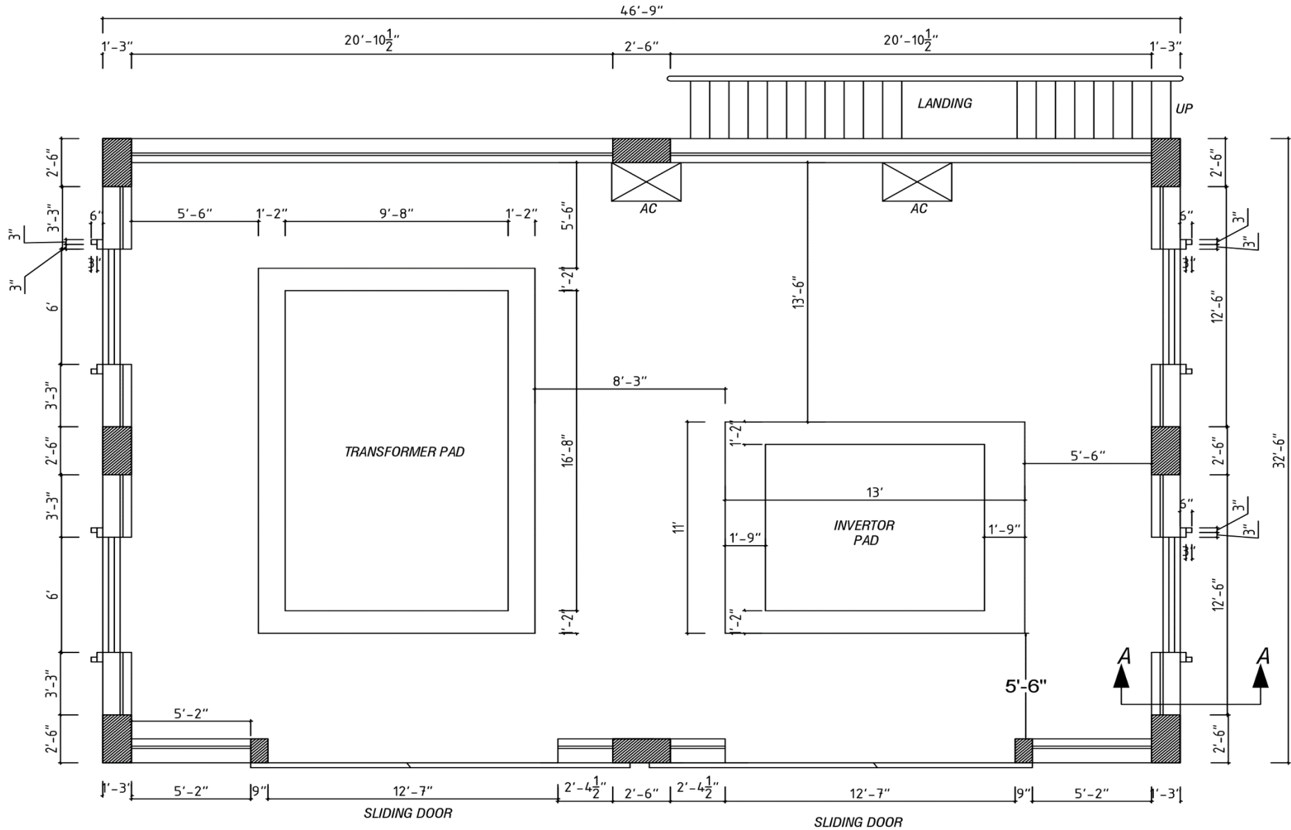
GROUND FLOOR WORKING (1519.375 square ft.)
